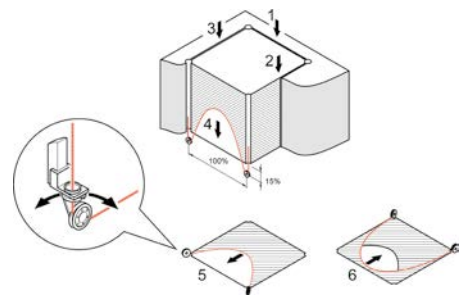
Immersion wire saw procedure for horizontal and vertical cutting. Cutting depths up to 2.5 m
