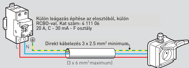
Green'UP Access 2 P+F aljzat
